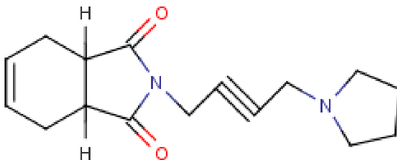
AM-6: 2-[4-(pyrrolidin-1-yl)but-2-yn-1-yl]-2,3,3a,4,7,7a-hexahydro-1H-isoindole-1,3-dione
