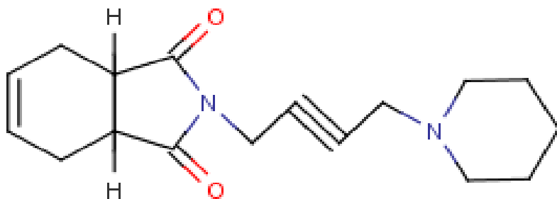
AM-4: 2-[4-(piperidin-1-yl)but-2-yn-1-yl]-2,3,3a,4,7,7a-hexahydro-1H-isoindole-1,3-dione
