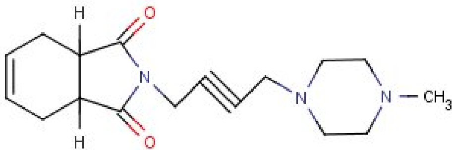
AM-5: 2-[4-(4-methylpiperazin-1-yl)but-2-yn-1-yl]-2,3,3a,4,7,7a-hexahydro-1H-isoindole-1,3-dione
